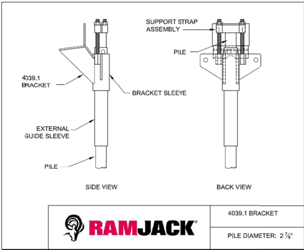
FIGURE 5—4039.1 SUPPORT BRACKET AND PILING
