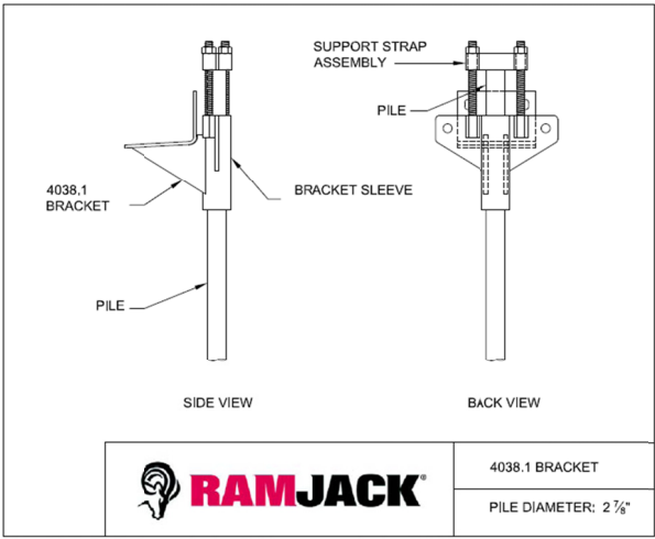
FIGURE 4—4038.1 SUPPORT BRACKET AND PILING
