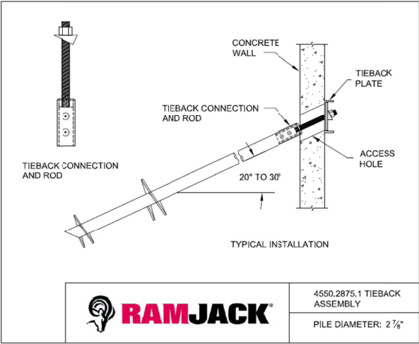
FIGURE 8—4550.2875.1 TIEBACK ASSEMBLY
