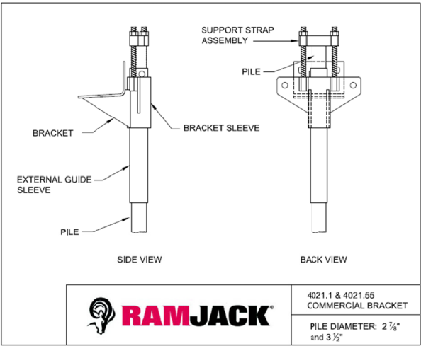
FIGURE 3—4021.1 and 4021.55 SUPPORT BRACKET ASSEMBLY
