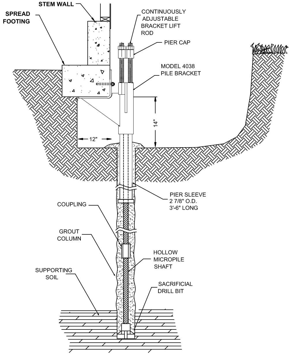
TYPICAL MICROPILE INSTALLATION NOT TO SCALE
