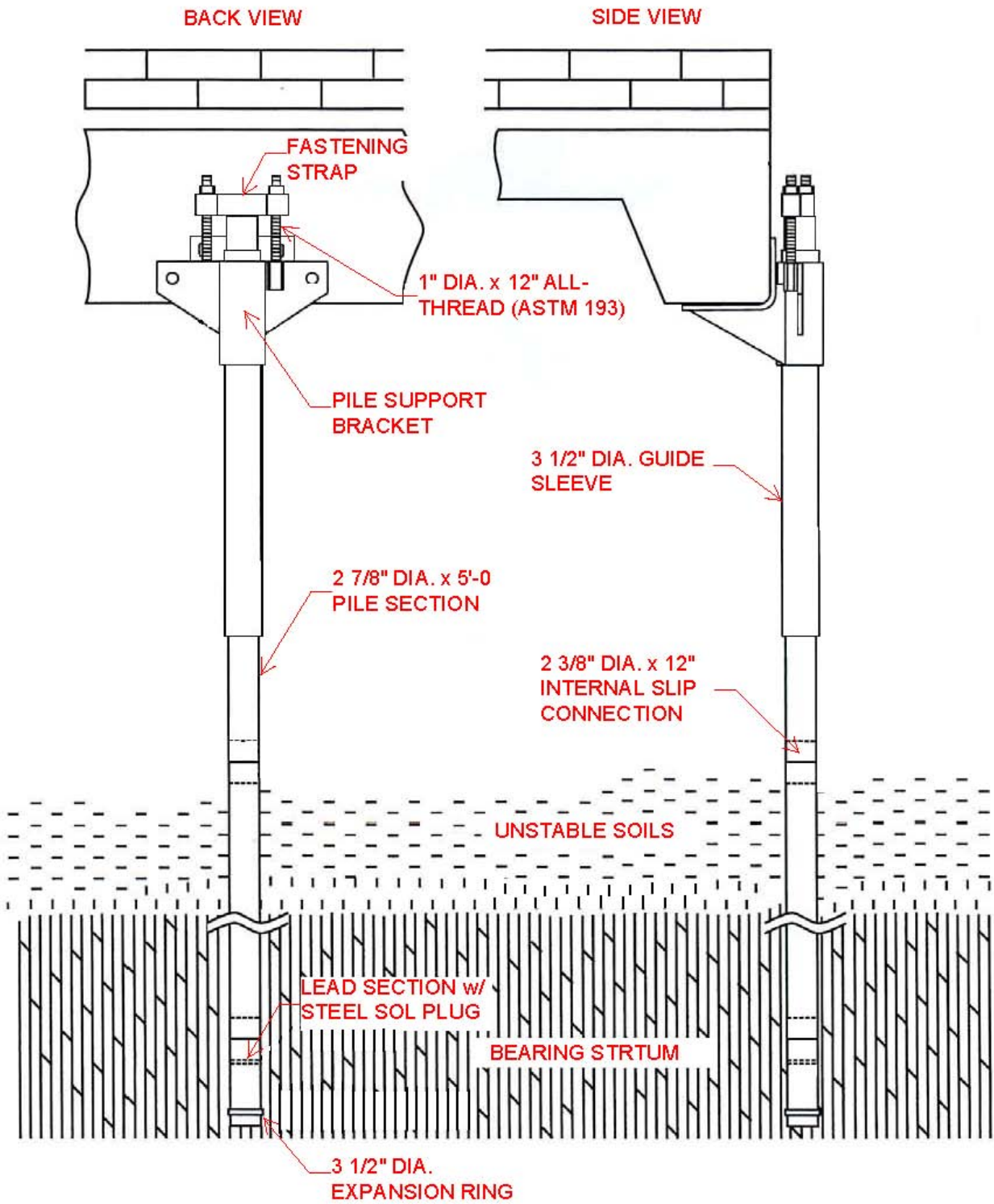
FIGURE 1 HYDRAULICALLY DRIVEN STEEL PILE ASSEMBLY SECTION DETAIL
