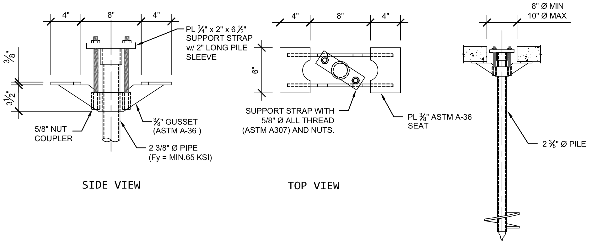
TYPICAL INSTALLATION DETAIL
